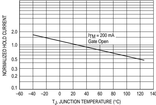
FIGURE 5 – HOLD CURRENT
