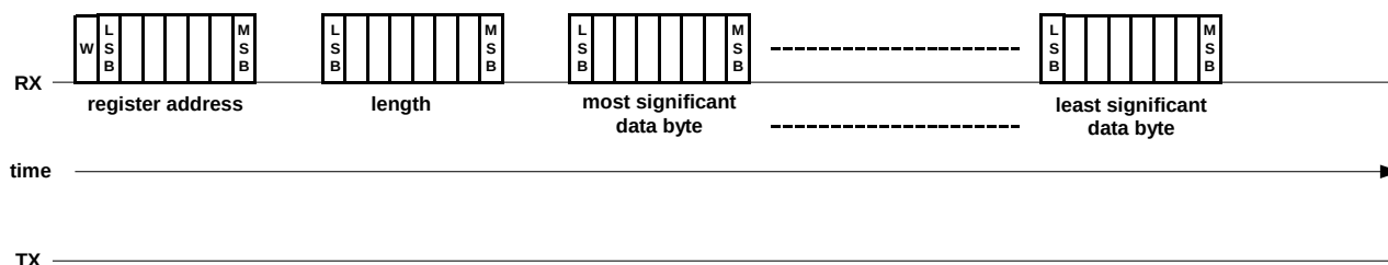
Figure 9: UART Write Operation
