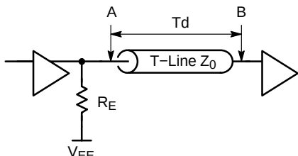
Figure 3. Unterminated Transmission Line Stub
