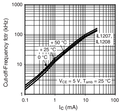
Fig. 17 - Cut-Off-Frequency (-3 dB) vs. Collector Current
