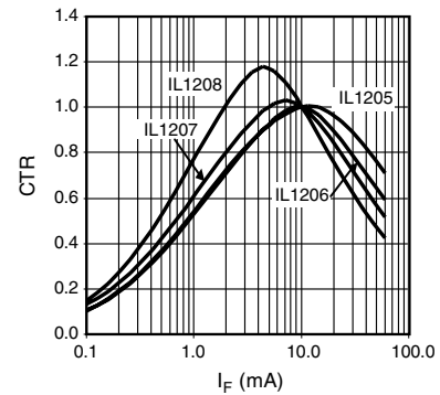
Fig. 13 - CTR vs. I_F Saturated, Normalised to I_F = 10\text{ mA} , T_{amb} = 25\text{ °C}
