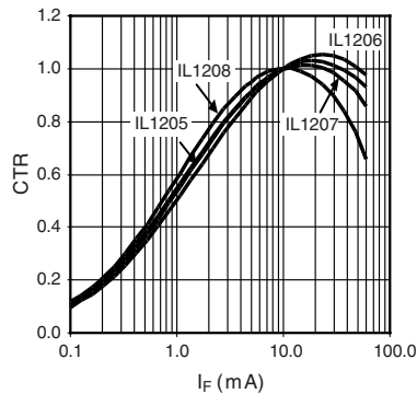
Fig. 11 - CTR vs. I_F , ( V_{CE} = 5\text{ V} , T_{amb} = 25\text{ °C} ) Normalised to I_F = 10\text{ mA} , T_{amb} = 25\text{ °C}
