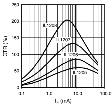
Fig. 12 - CTR vs. I_F Saturated, ( V_{CE} = 0.4\text{ V} , T_{amb} = 25\text{ °C} )
