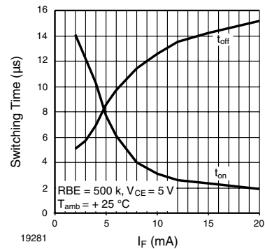
Fig. 20 - Switching Time vs. I_F
