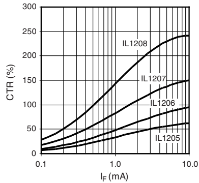
Fig. 10 - CTR vs. I_F , ( V_{CE} = 5\text{ V} , T_{amb} = 25\text{ °C} ) (Not Normalised)
