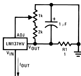
Figure 8. Current Regulator
