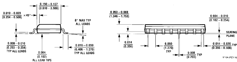
16-Lead Small Outline Molded Package (M) Order Number DM74LS138M or DM74LS139M Package Number M16A
