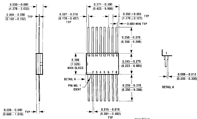
16-Lead Ceramic Flat Package (W) Order Number 54LS138FMQB, 54LS139FMQB, DM54LS138W or DM54LS139W Package Number W16A
