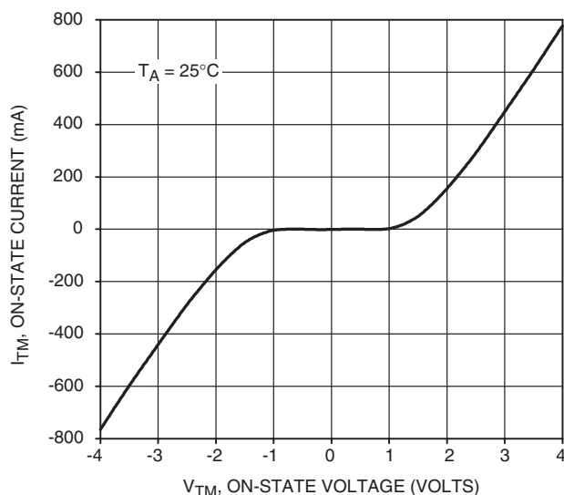
Figure 6. On-State Characteristics
