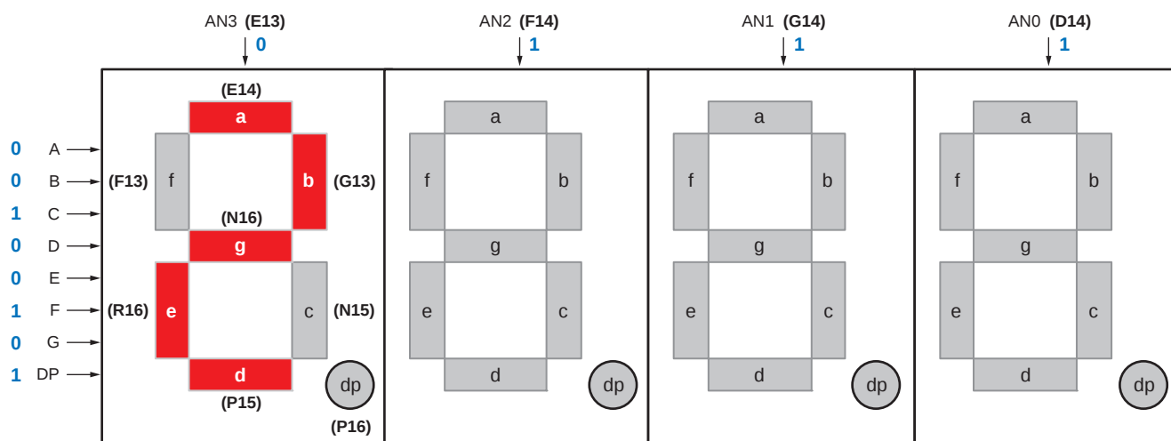
Figure 3-1: Seven-Segment LED Digit Control
