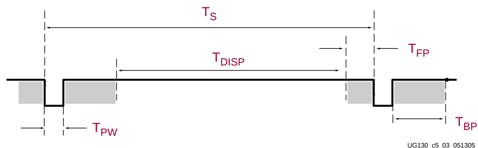
Figure 5-3: VGA Control Timing
