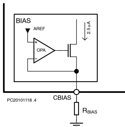
Figure 10. Bias Circuit
