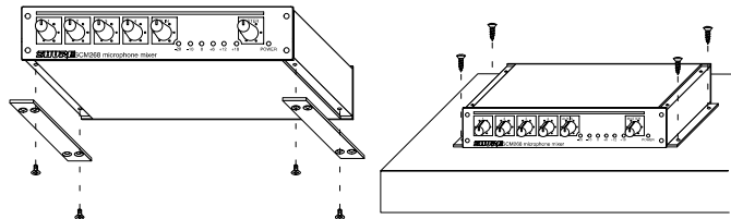
TOP MOUNT
