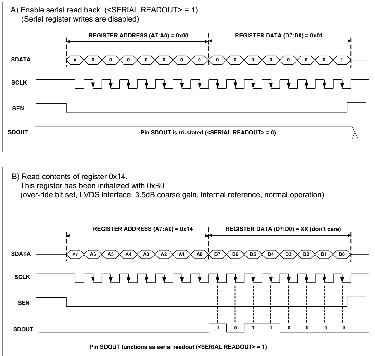
Figure 7. Serial Readout
