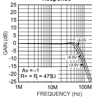
Closed-Loop Frequency Response
