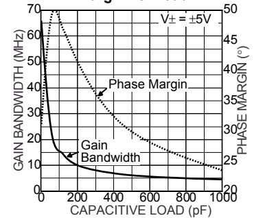
Gain Bandwidth and Phase Margin vs. Load
