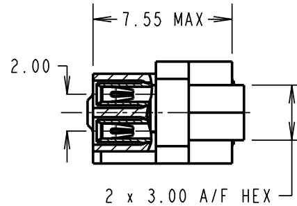
PART SECTION X-X
