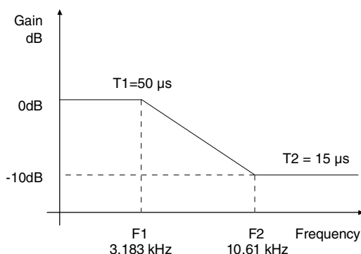
Figure 35. De-Emphasis Curve
