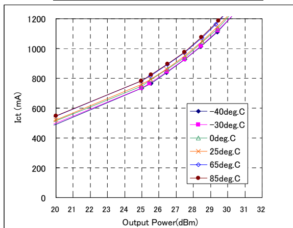
Operating Current vs. Output Power
