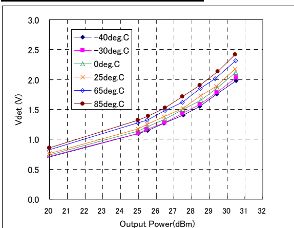
Detector Voltage vs. Output Power
