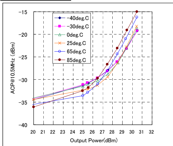
ACP Characteristics
