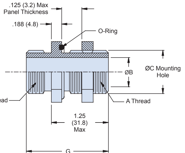
Bulkhead Feed-Throughs 710-102/103/373
