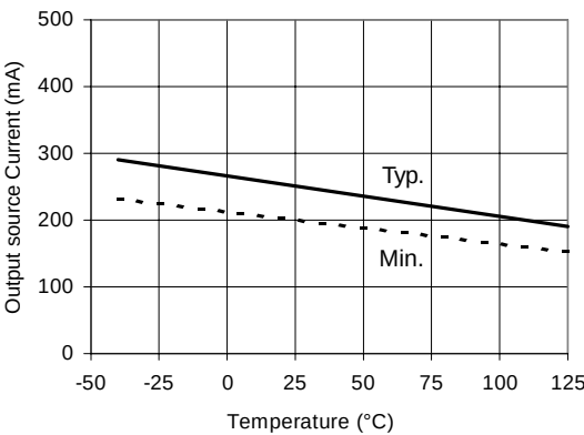
Figure 29A Output Source Current vs Temperature
