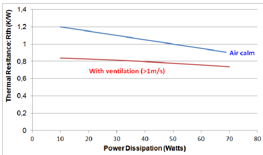
Performances thermiques en montage vertical Thermal performances in vertical mounting
