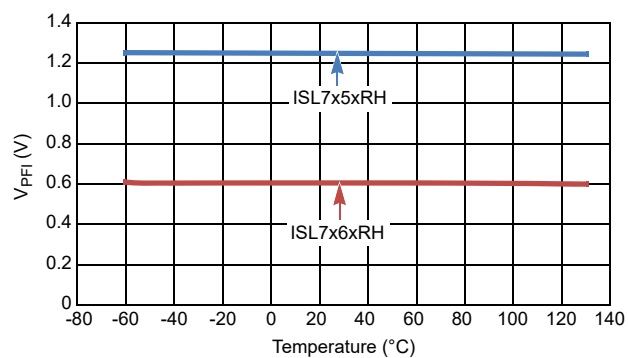
Figure 8. V_{PFI} vs Temperature
