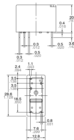
1 Form C
