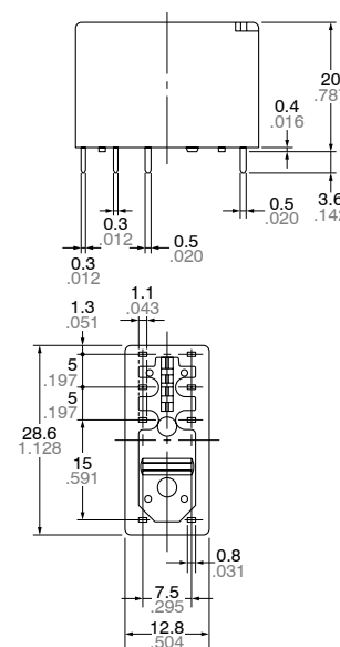
2 Form C
