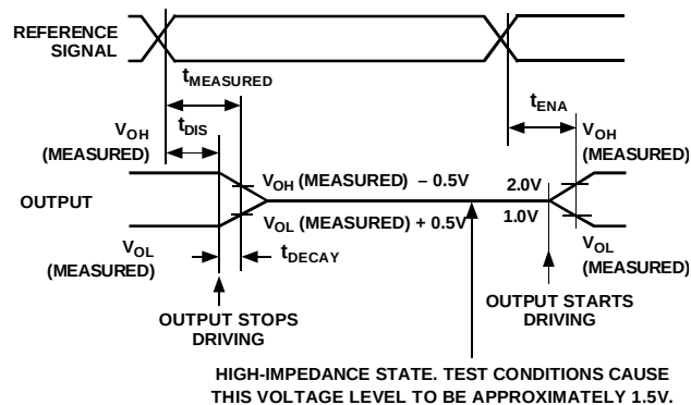
Figure 18. Output Enable/Disable
