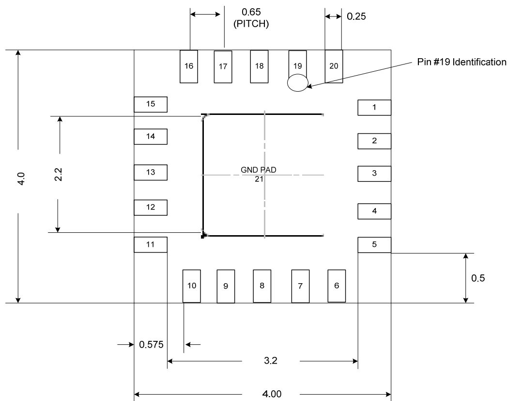
BOTTOM VIEW
