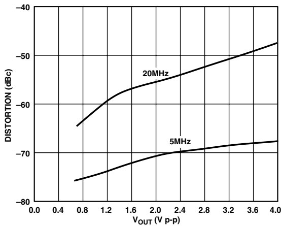
TPC 21. Distortion vs. V_{OUT} @ 20 MHz, 5 MHz, R_L = 150\Omega , V_S = \pm 5.0V
