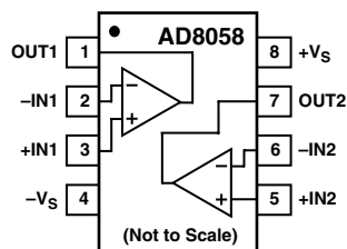
RM-8 (MSOP) R-8 (SOIC)
