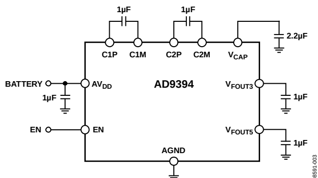
Figure 4. Application Schematic
