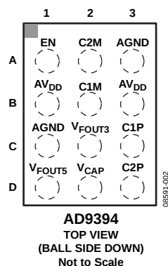
Figure 2. Pin Configuration
