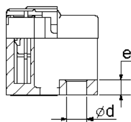
B-B (1:1)
