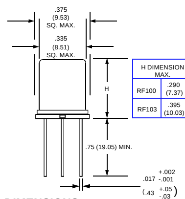
EXTERNAL DIMENSIONS
