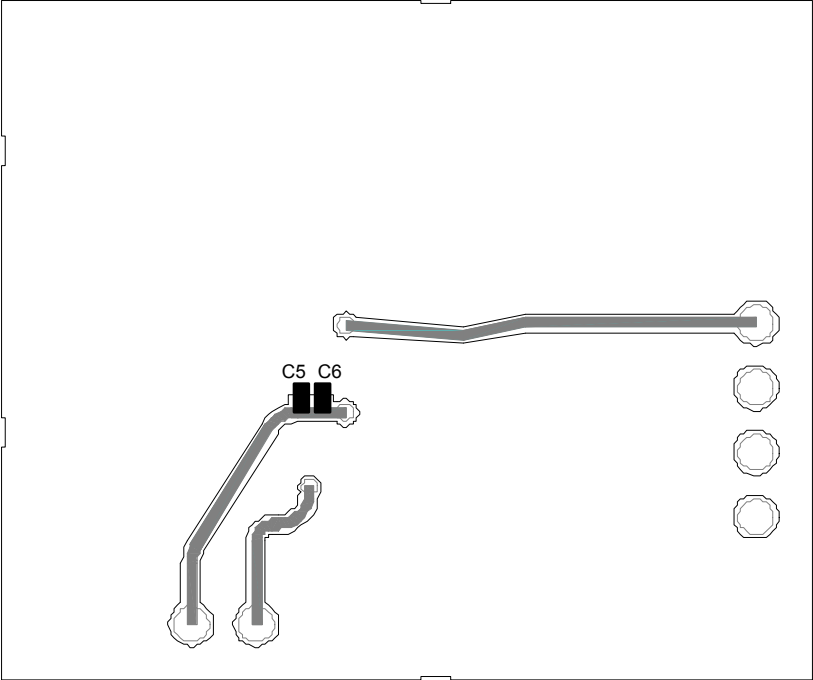
Figure 15. Back Side
