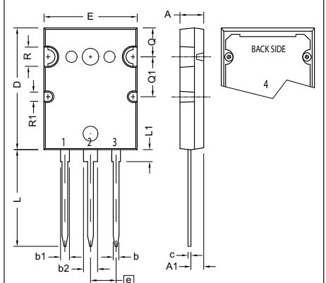
X021a PLUS264™ Weight = 10 g
