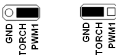
Figure 4. TORCH Jumper Settings
