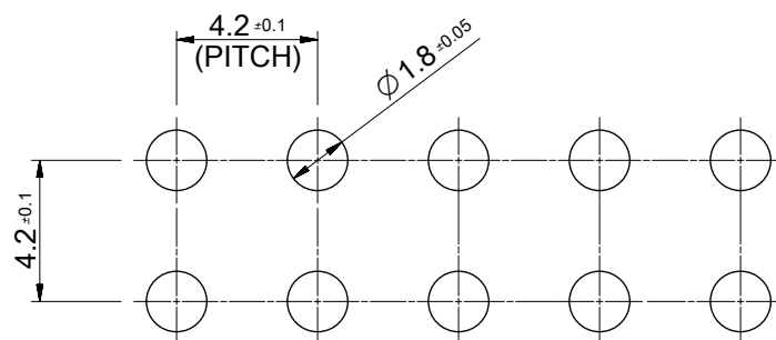
RECOMMENDED P.C. BOARD PATTERN
