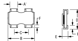
CAY16-J2
