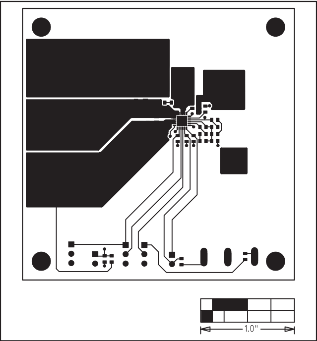
Figure 3. MAX15038 EV Kit PCB Layout—Component Side
