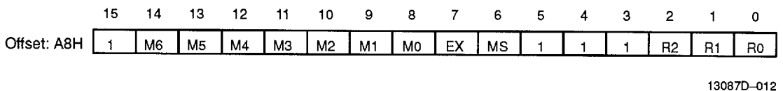
Figure 11. MPCS Register
