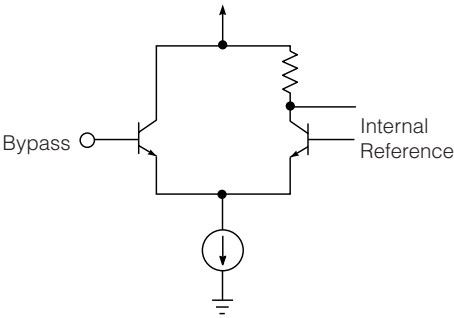
Figure 8 Bypass Circuit
