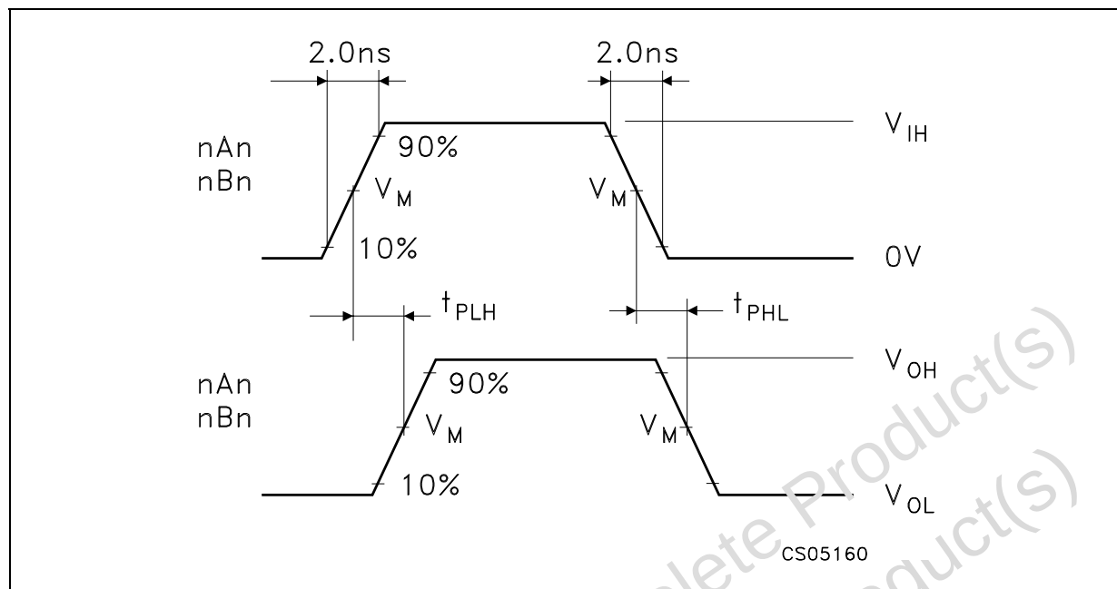
WAVEFORM 1: PROPAGATION DELAYS ( f=1\text{MHz} ; 50% duty cycle)
