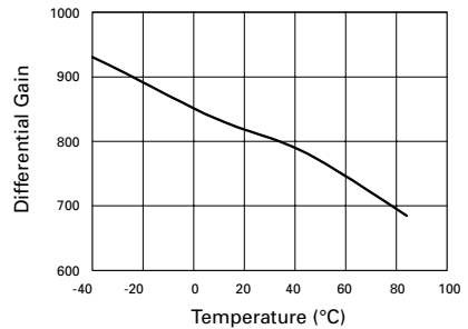
AUX Open Loop Gain V Temp.
