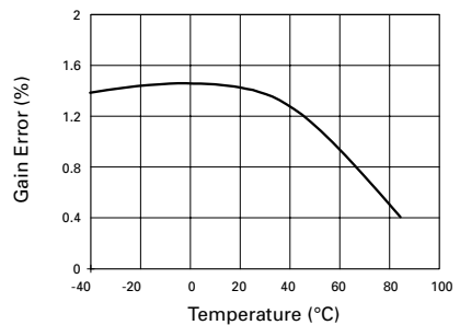
LOG/REC Gain Error V Temp.
