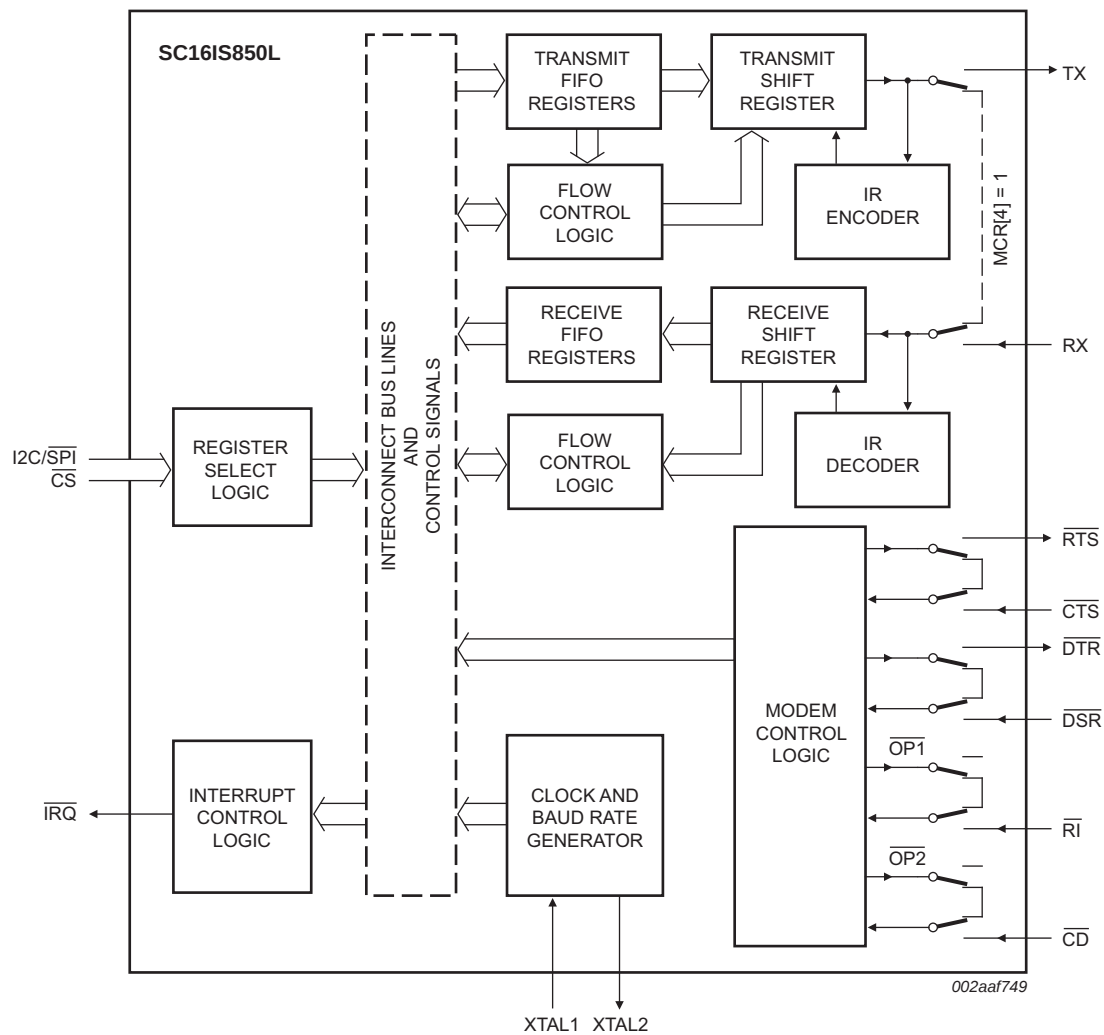
Fig 8. Internal Loopback mode diagram
