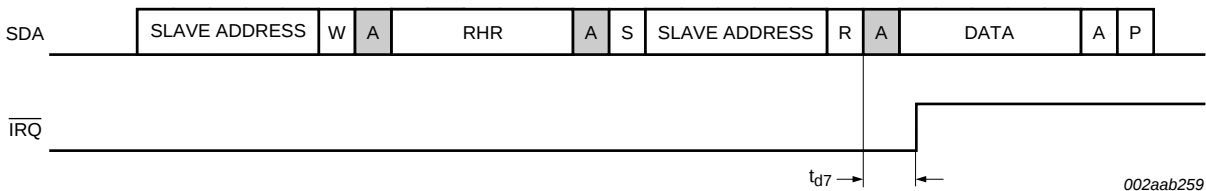
Fig 22. Receive interrupt clear
