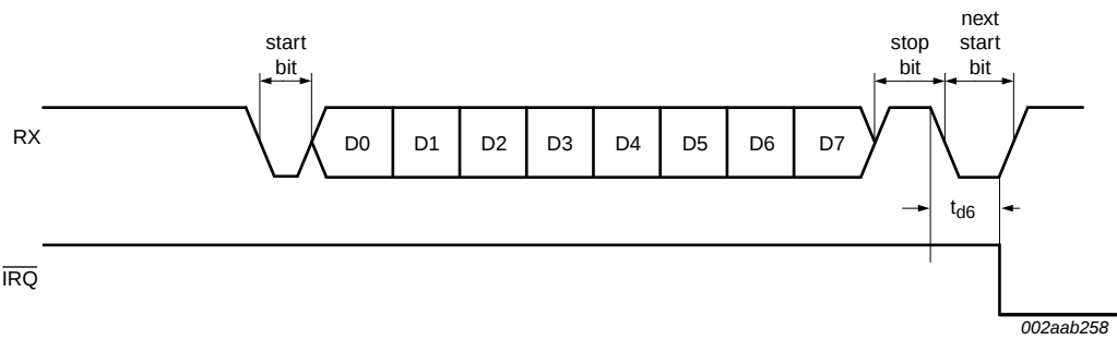
Fig 21. Receive interrupt
