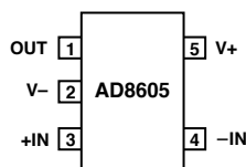
5-Lead SOT-23 (RT Suffix)
