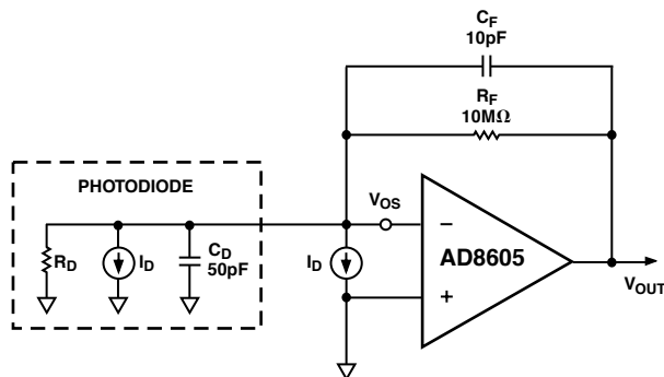
Figure 8. Equivalent Circuit for Photodiode Preamp
