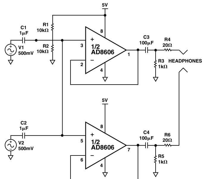
Figure 9. Single-Supply Headphone/Speaker Amplifier
