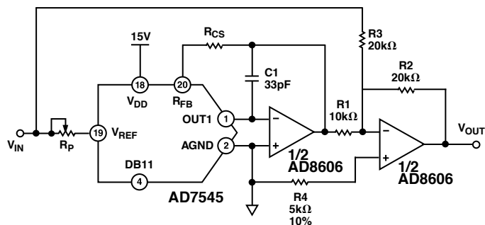
Figure 12. Bipolar Operation
