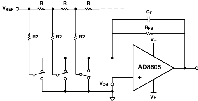
Figure 11. Simplified Circuit of the DAC8143 with AD8605 Output Buffer
