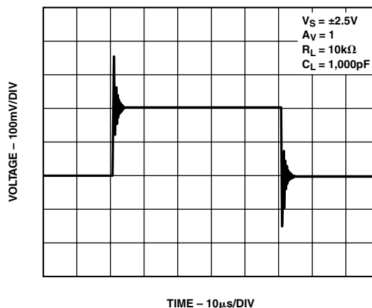
Figure 5. Capacitive Load Drive without Snubber
