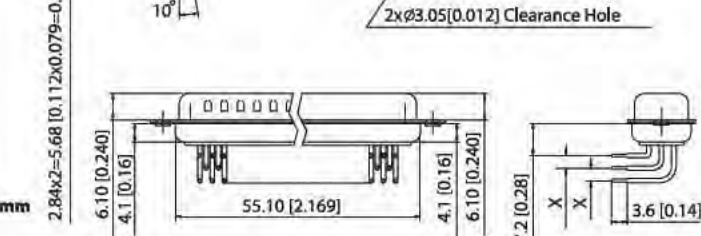
50 Positions Machined Pin (W/O Rear Cover)
