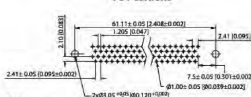
78 Positions
