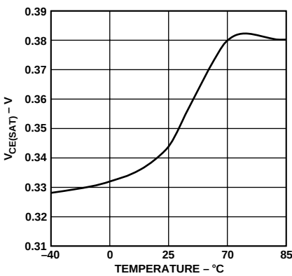
Figure 10. Switch Saturation Voltage vs. Temperature
