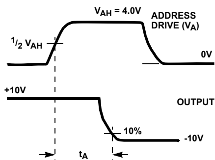
FIGURE 6C. MEASUREMENT POINTS
