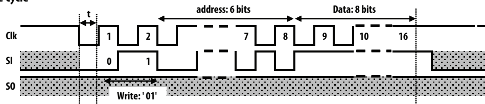
Figure 6. SPI timing diagram for read and write
