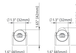
Clip mount end view
