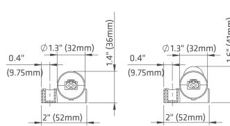
Screw mount end view
