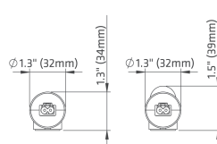
Magnet mount end view
