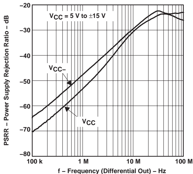
POWER SUPPLY REJECTION RATIO vs FREQUENCY (DIFFERENTIAL OUT)
