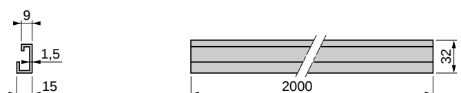
Asymmetrical rails DZ5-MB201
