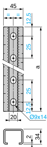
Pre-drilled notched uprights AM3-EC●●●
