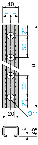
Combination rails AM1-ED0●1
