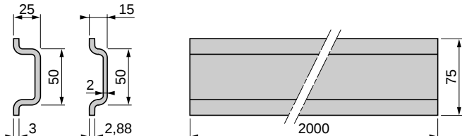
Omega" mounting rail AM1-DL200, DL201, Common front face view
