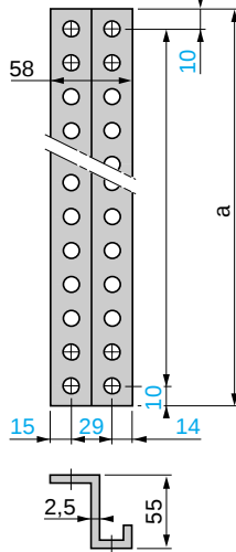
Pre-drilled uprights DZ6-MZ●●●
