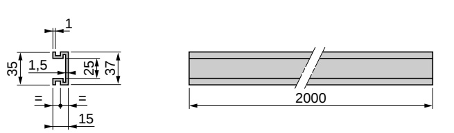
Aluminium mounting rail AM1-EA200
