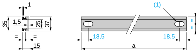
Combination rails AM1-ED●●5
