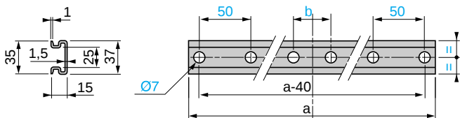
Combination rail AM1-ED201
