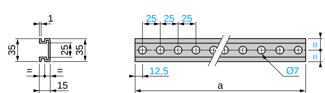
Combination rails AM1-ED200
