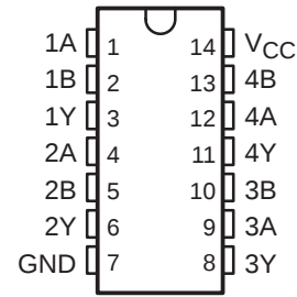
SN54HCT08 . . . J OR W PACKAGE SN74HCT08 . . . D, DB, N, OR PW PACKAGE (TOP VIEW)
