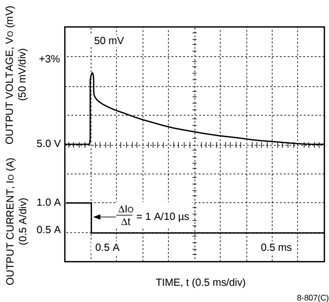
Figure 10. MK010 Typical Output Voltage Waveform for a Step Load Change from 50% to 25% of I_{O, max} ; V_I = 48 \text{ V} ; T_A = 25^\circ \text{C}
