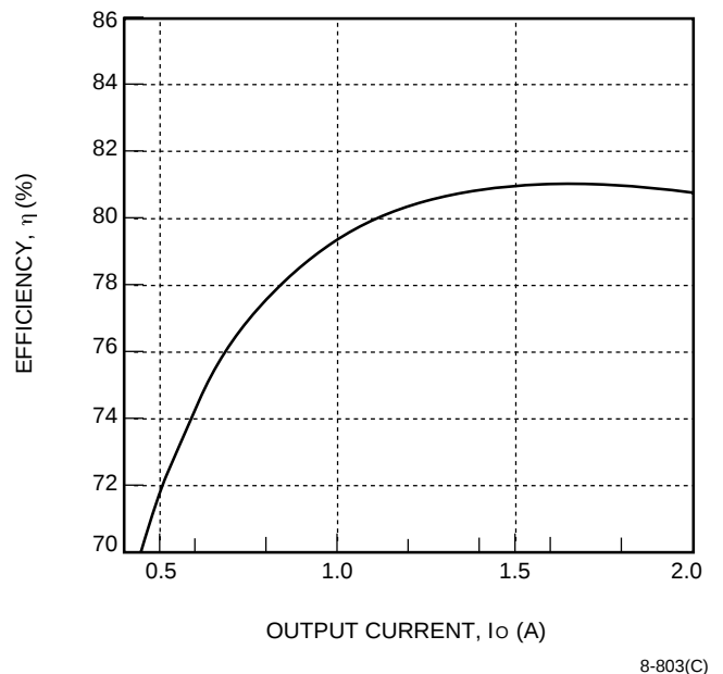
Figure 8. MK010A1, N1 Typical Converter Efficiency as a Function of Output Current; V_I = 48 V; T_A = 25 °C
