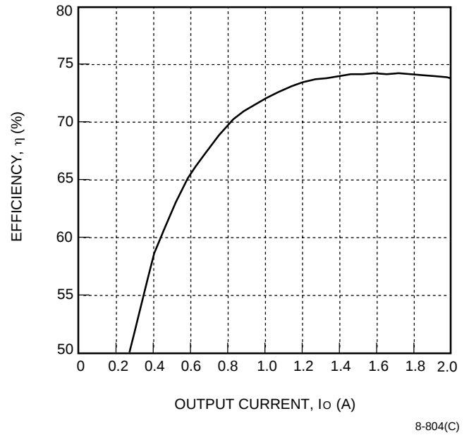
Figure 7. MK010F1 Typical Converter Efficiency as a Function of Output Current; V_I = 48 V; T_A = 25 °C
