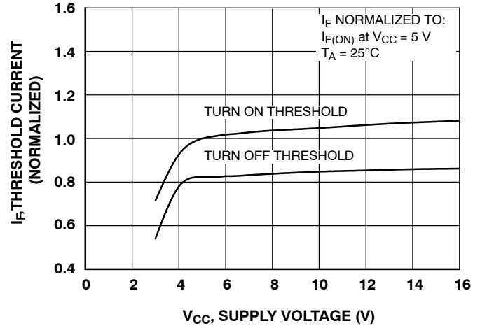
Figure 2. Threshold Current vs. Supply Voltage
