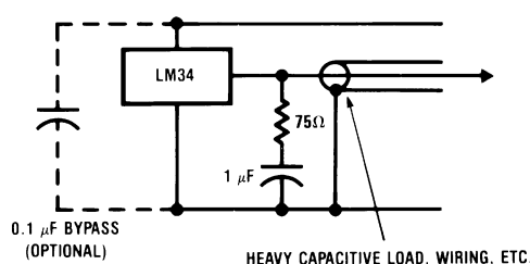
Figure 13. LM34 With R-C Damper
