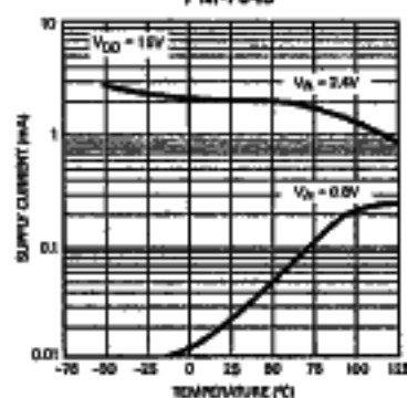
SUPPLY CURRENT vs TEMPERATURE PM-7645
